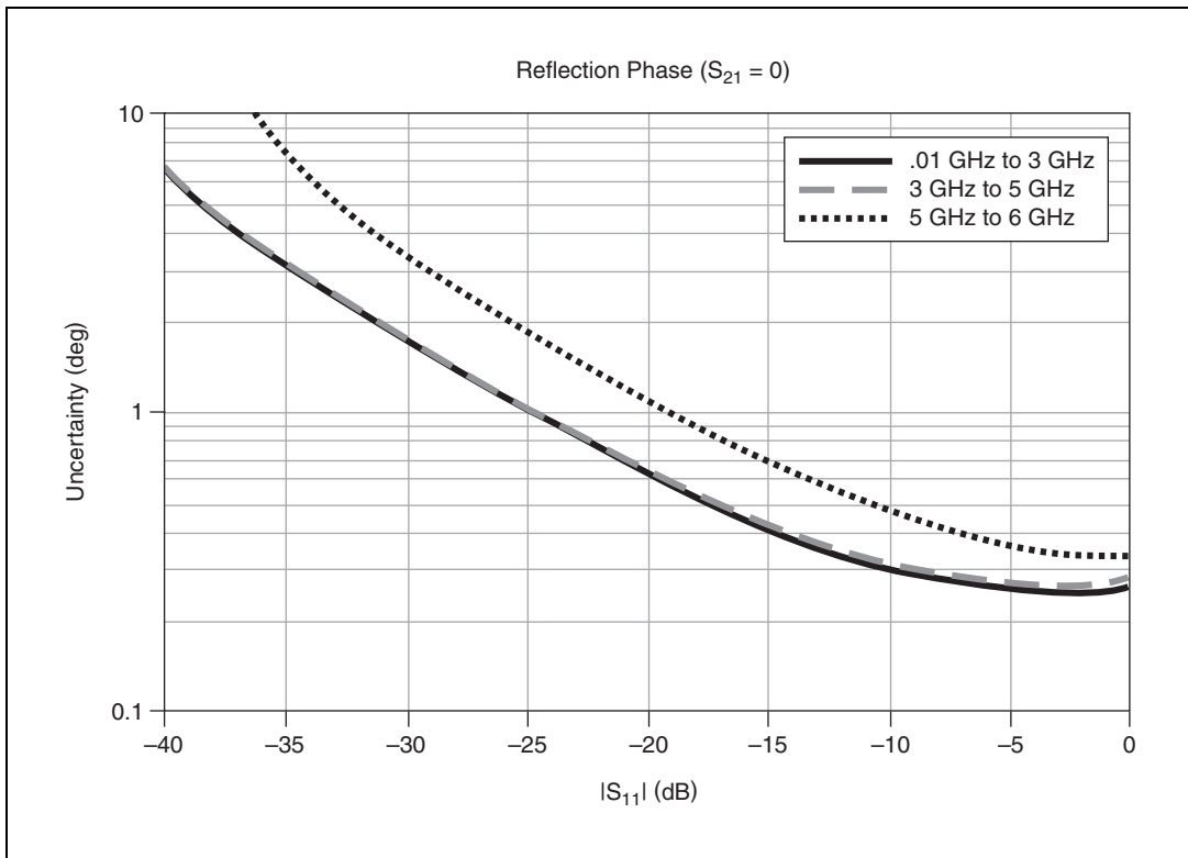
Figure 4. Phase Uncertainty
