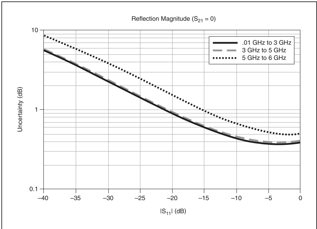
Figure 11. Magnitude Uncertainty
