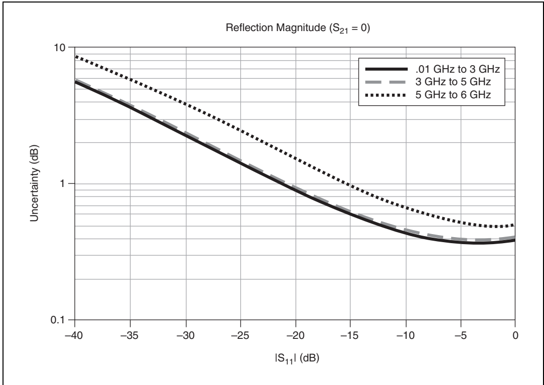
Figure 3. Magnitude Uncertainty
