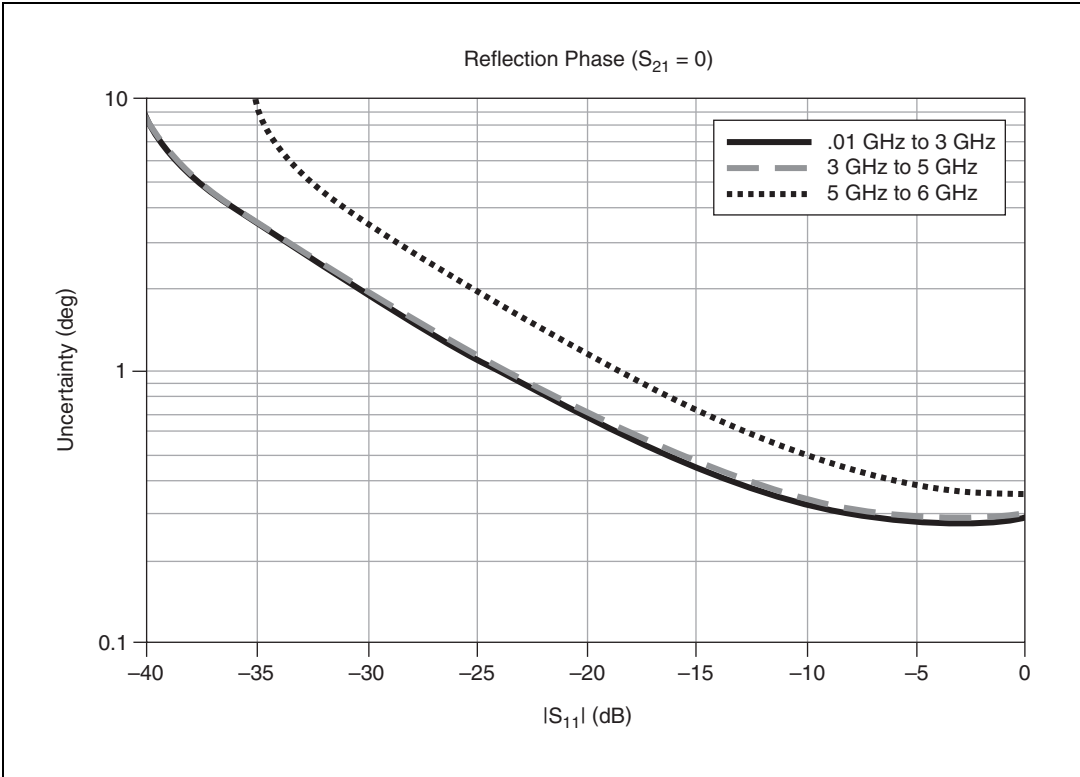
Figure 8. Phase Uncertainty
