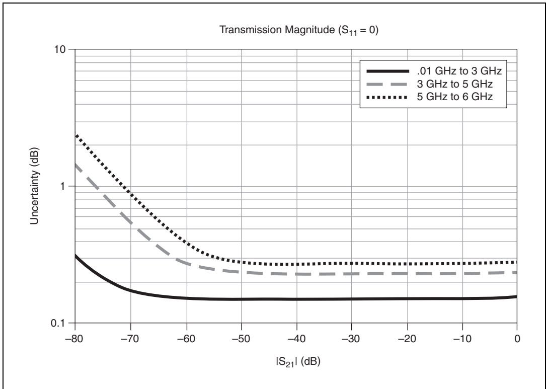
Figure 9. Magnitude Uncertainty
