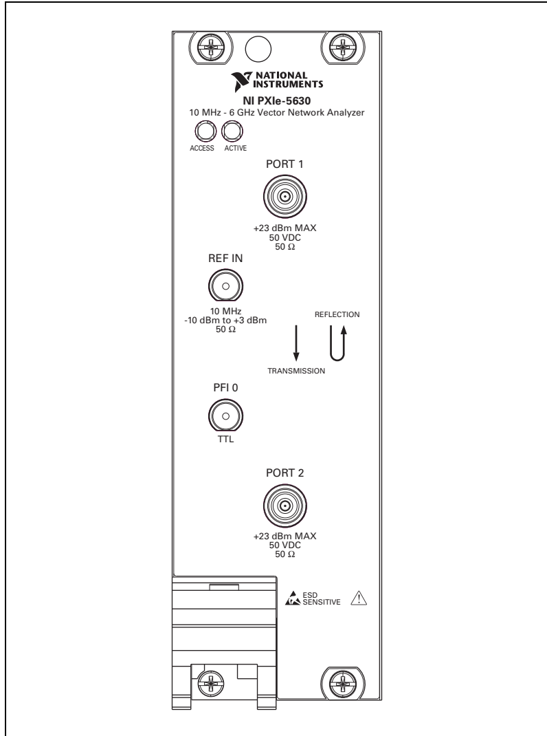
Figure 13. NI 5630 Front Panels
