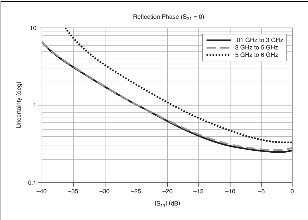
Figure 12. Phase Uncertainty
