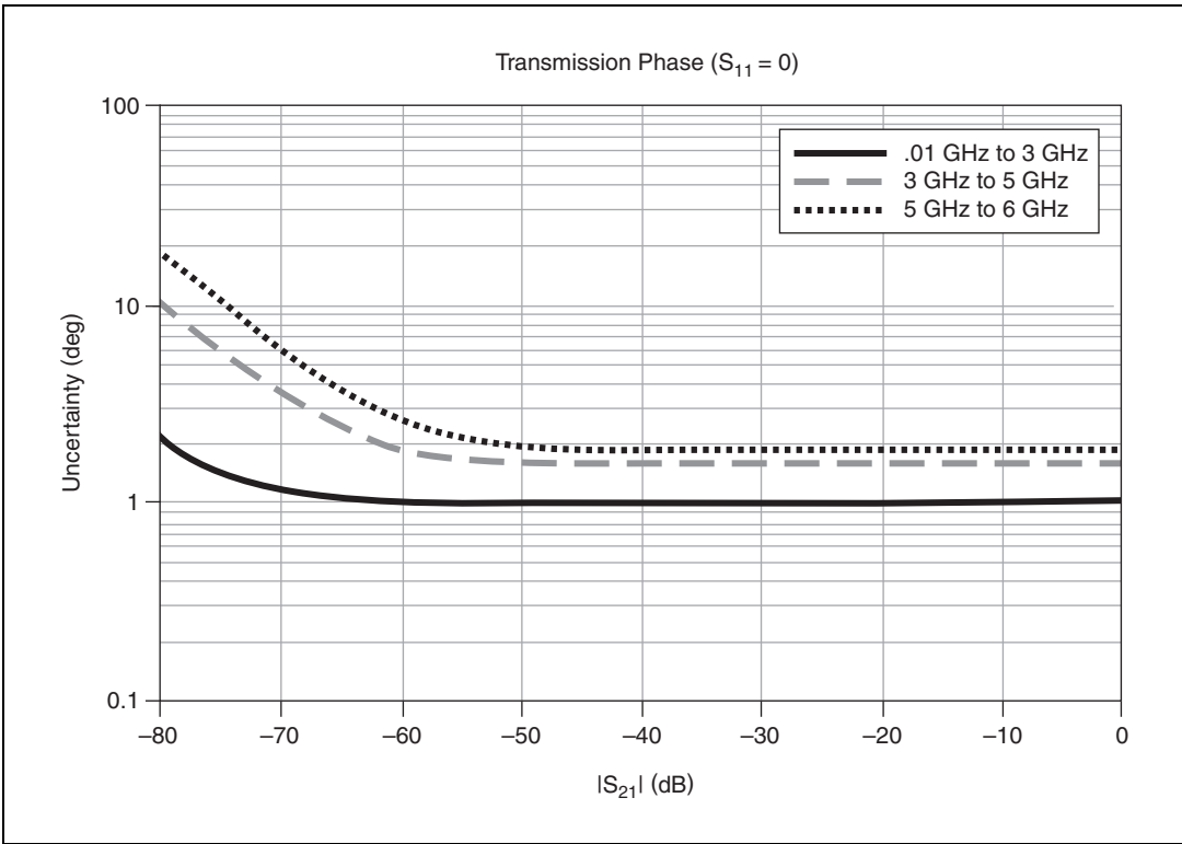
Figure 2. Phase Uncertainty
