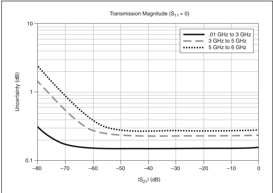
Figure 1. Magnitude Uncertainty
