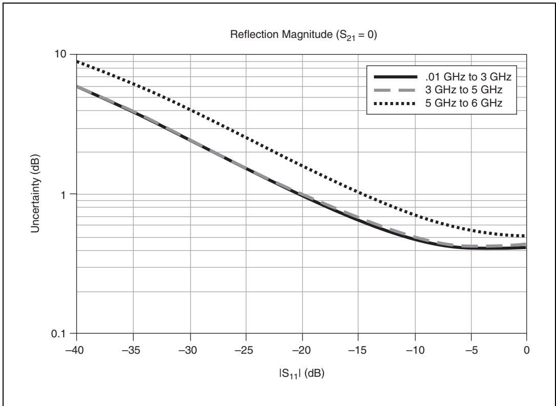
Figure 7. Magnitude Uncertainty
