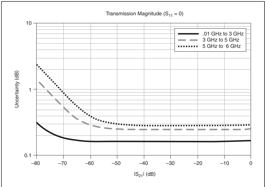
Figure 5. Magnitude Uncertainty
