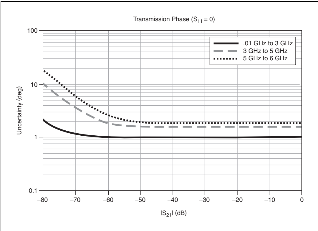
Figure 10. Phase Uncertainty
