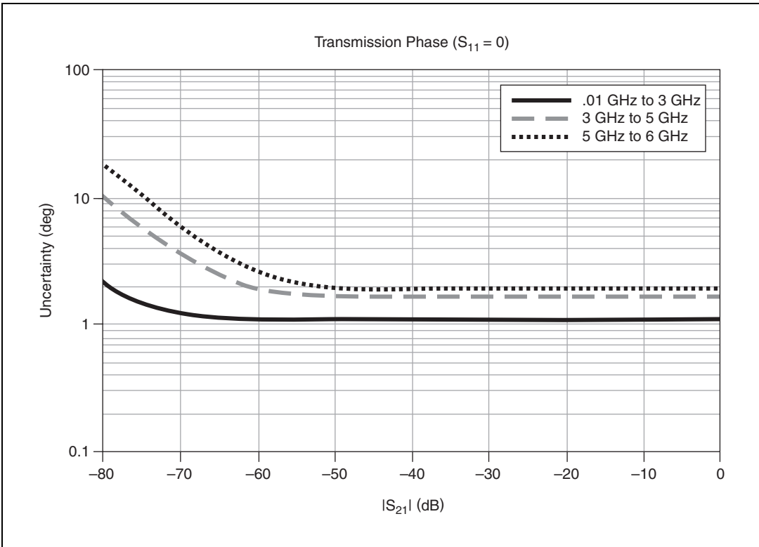
Figure 6. Phase Uncertainty
