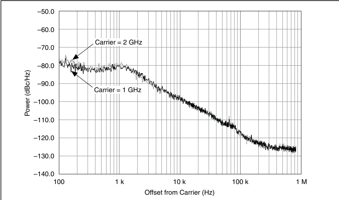
Figure 2. Typical Phase Noise at 1 GHz and 2 GHz, Instantaneous Bandwidth > 10 MHz
